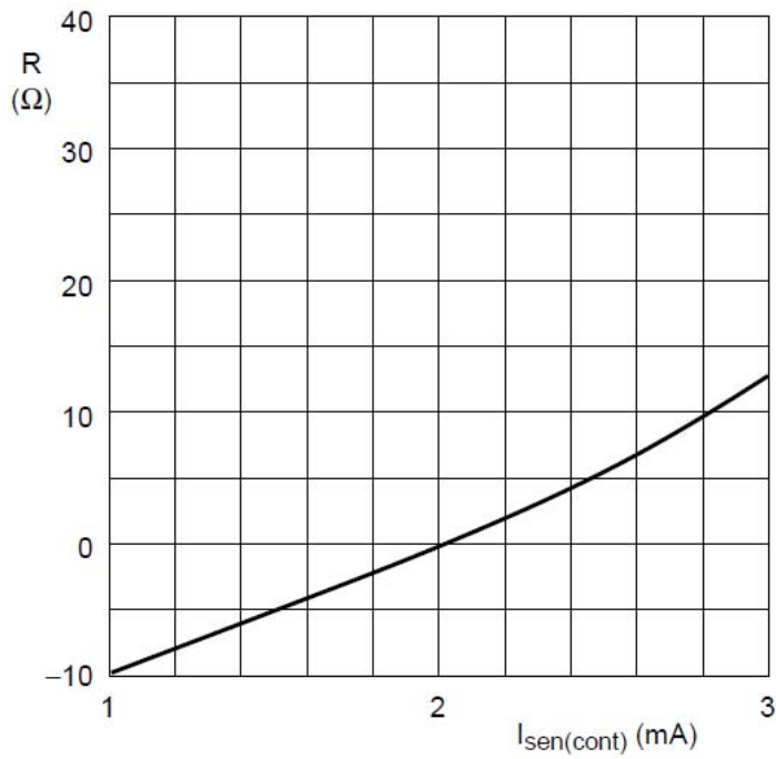
Fig 3. Deviation of sensor resistance as a function of operating current in still liquid
